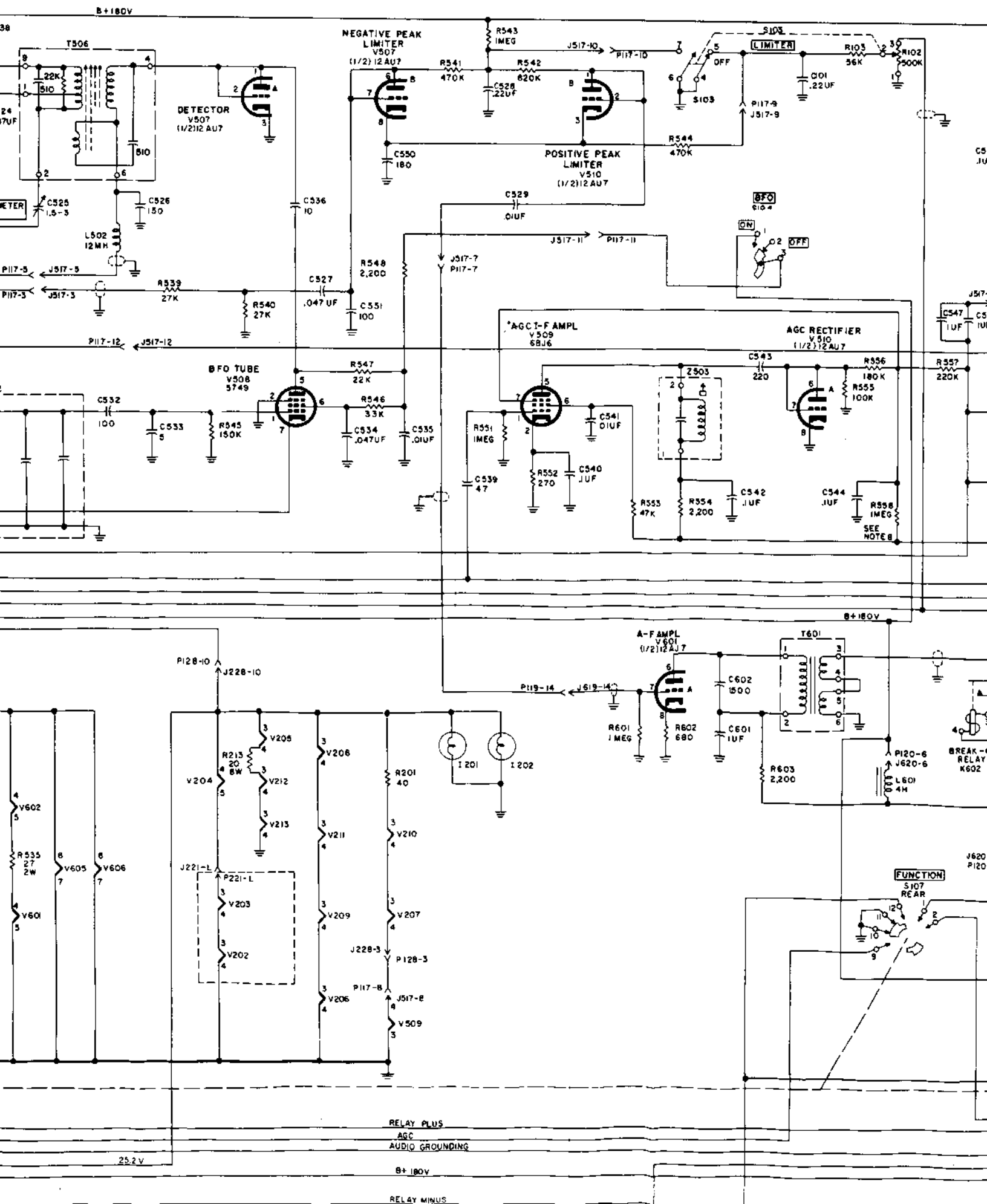
Figure 89. Radio Receiver R-388/URR, schematic diagram—Continued.
