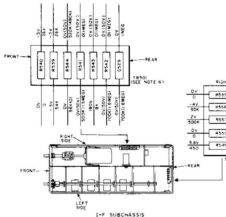
Figure 68. Voltages and resistances at terminal boards.
