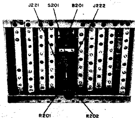
Figure 52. Section of rf subchassis, showing hand-switching mechanism.
