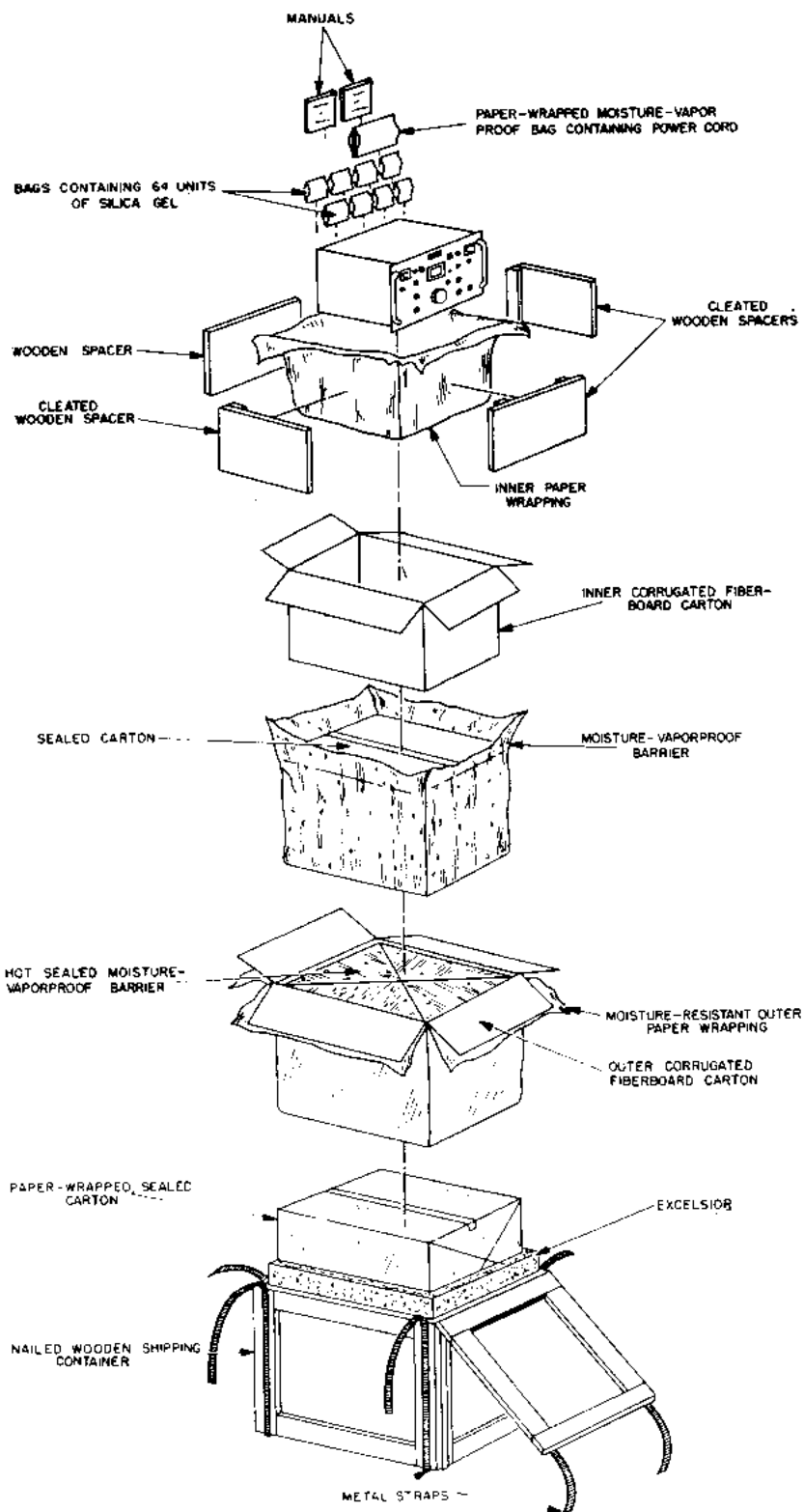
Figure 3. Packaging.
