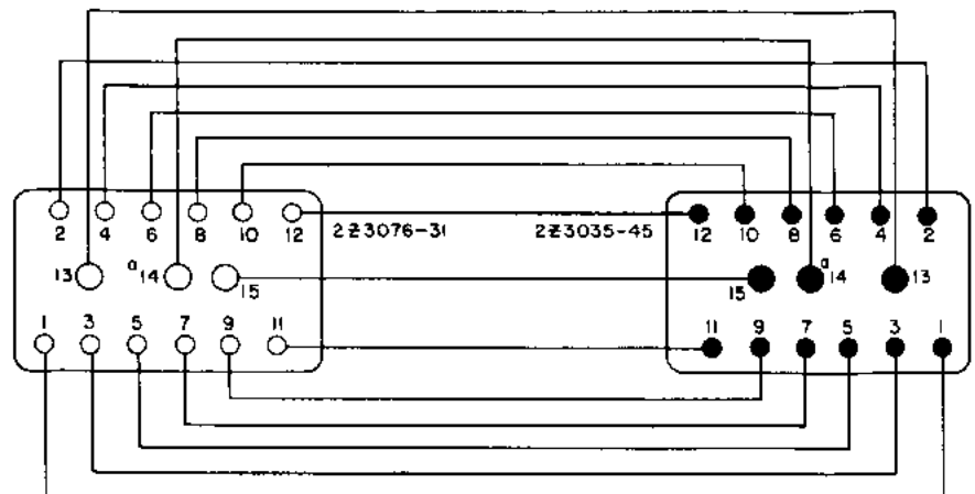
CABLE NO. 6
