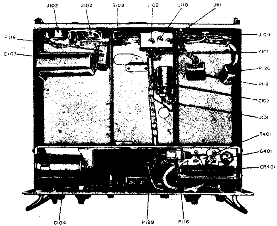
Figure 55. Front panel and main frame, bottom view.
