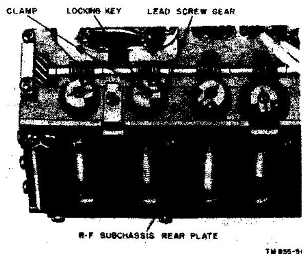
Figure 79. Sectional view of slug-rack lead screw drive assembly.
