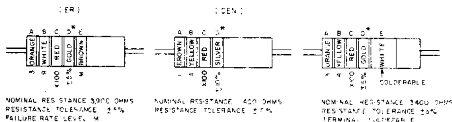
COMPOSITION-TYPE RESISTORS
