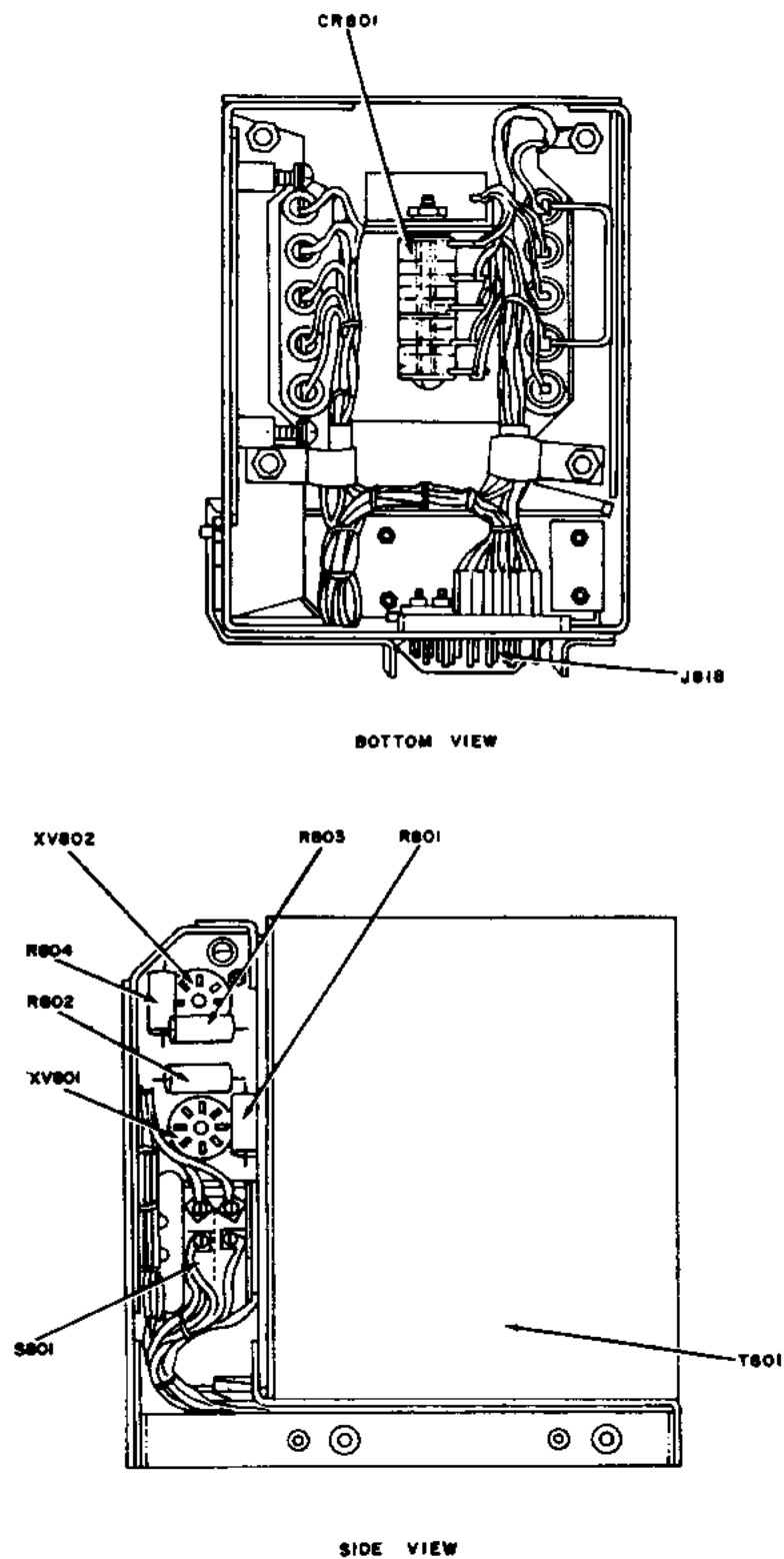
Figure 63. Power Supply PP-621/URR, bottom and side views.
