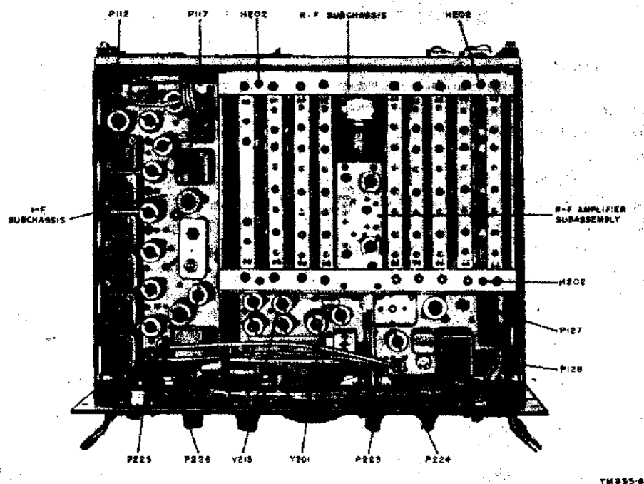
Figure 70. Top view, dust cover and shield removed.
