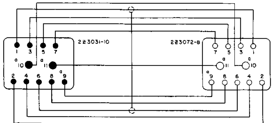
CABLE NO. 3
