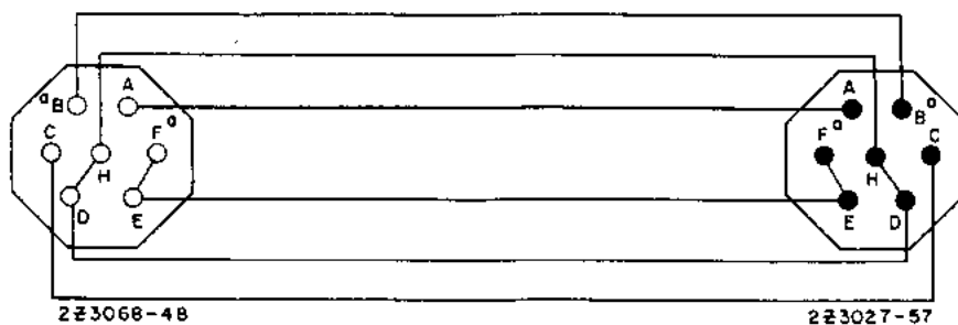
CABLE NO.7
