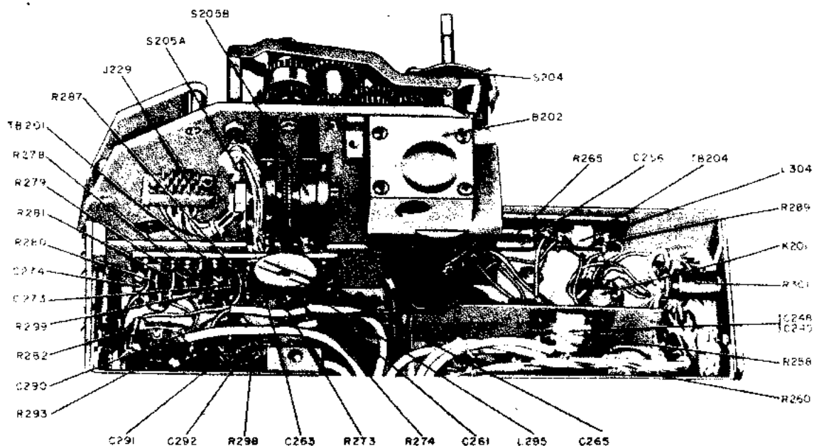
Figure 5a. Rf sub-chassis, bottom view, showing gears.
