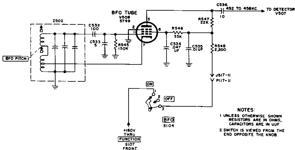
Figure 27. Bfo, schematic diagram.
