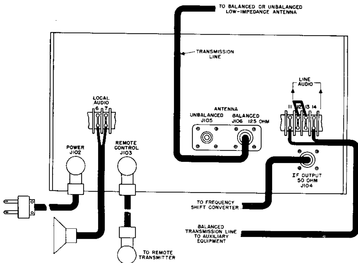
Figure 8. Cording diagram.
