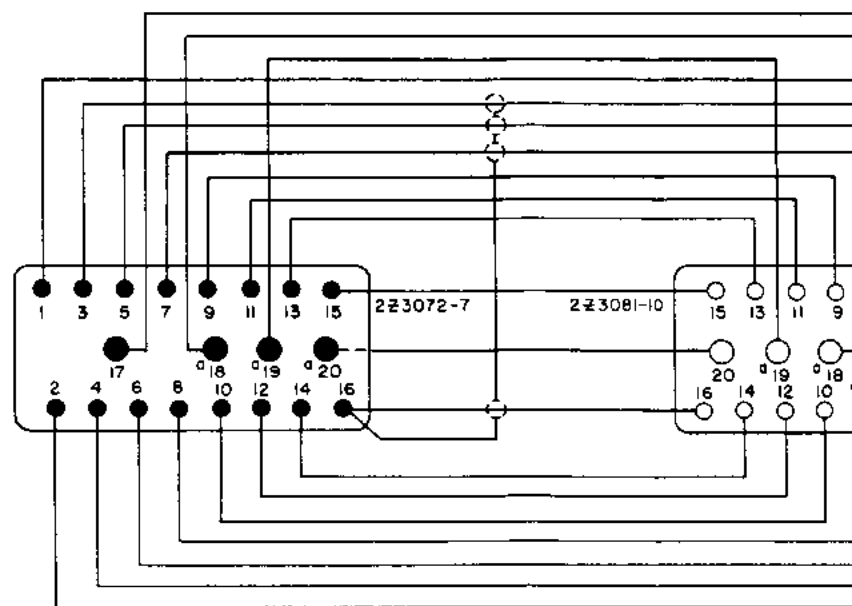
CABLE NO. 2
