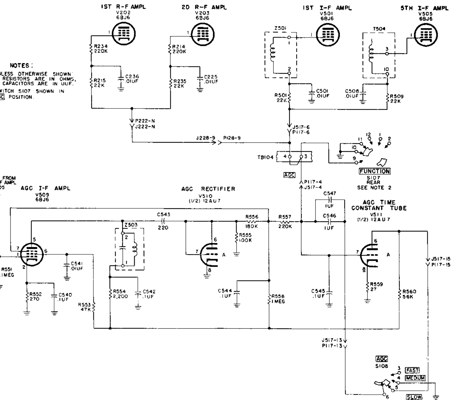
Figure 56. Age voltage distribution.
