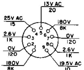
1ST MIXER V204 12AT7
