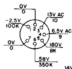
RELAY CONTROL V210 6C4W
