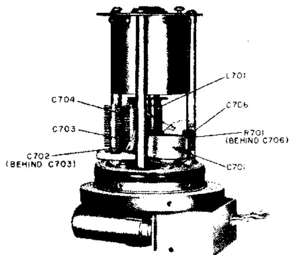
Figure 59. Vfo subchassis, cover and heating element removed.
