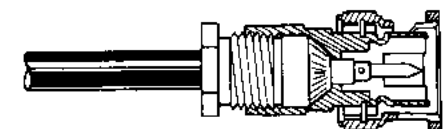
Figure 47. Assembly instruction for cables Nos. 1 and 1A.
