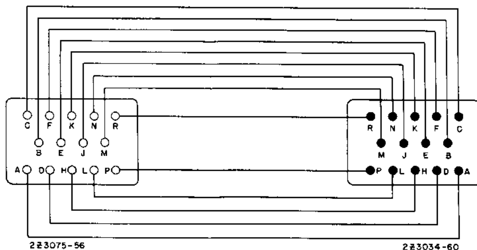
CABLE NO.4
