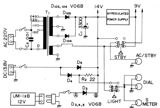
Power Supply
