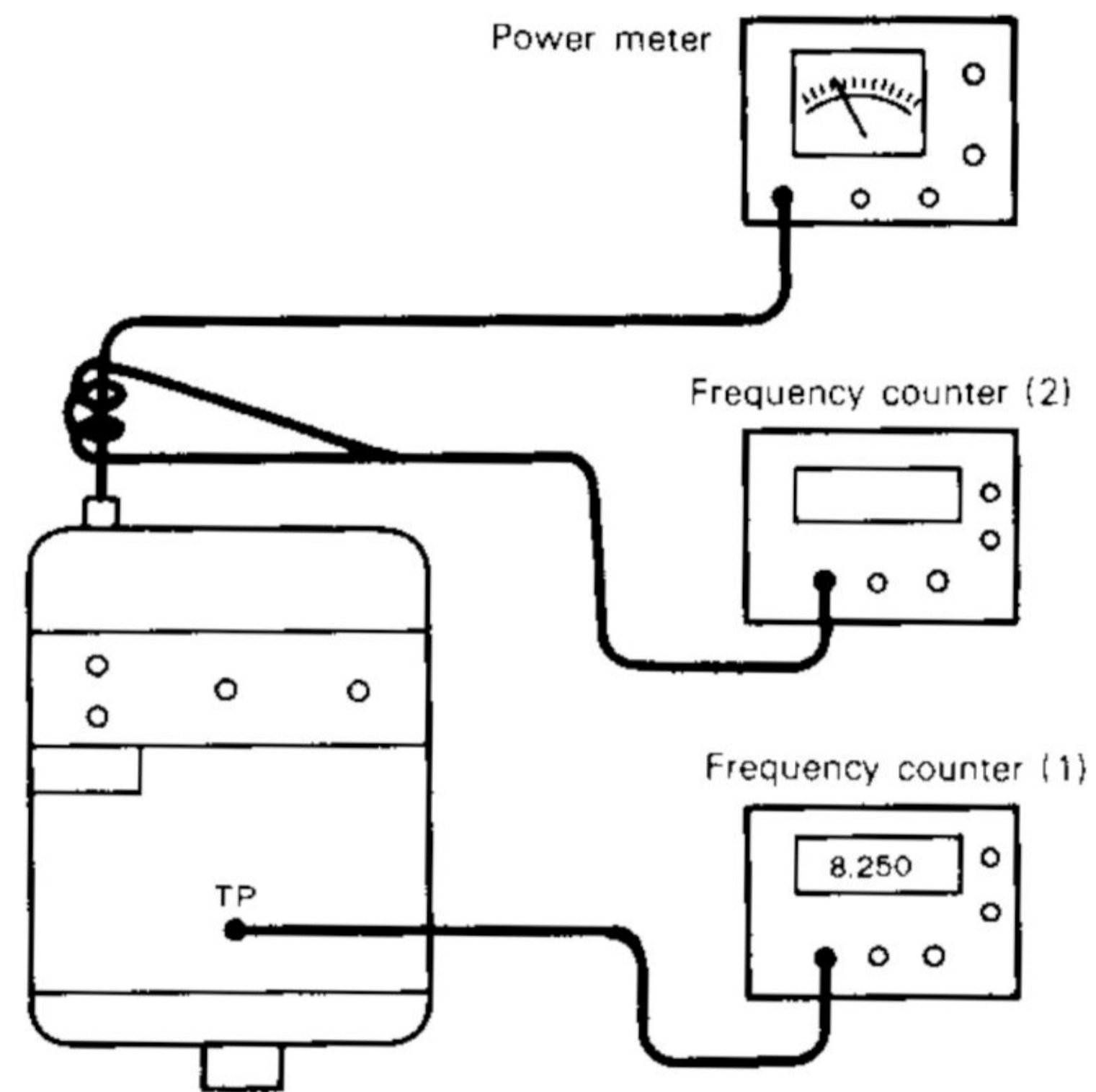
FIG. 19 FREQUENCY ADJUSTMENT
