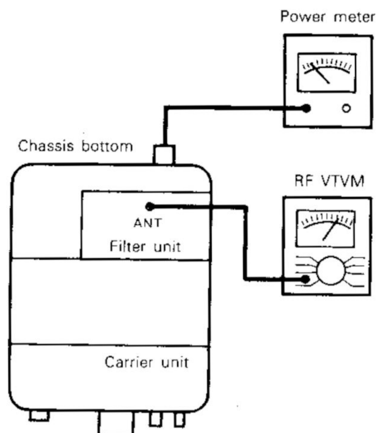
FIG. 11 ADJUSTMENT OF CARRIER SUPPRESSION
