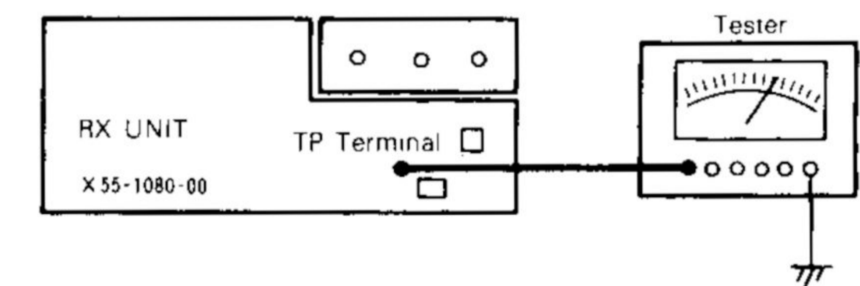
FIG. 17 NB ADJUSTMENT
