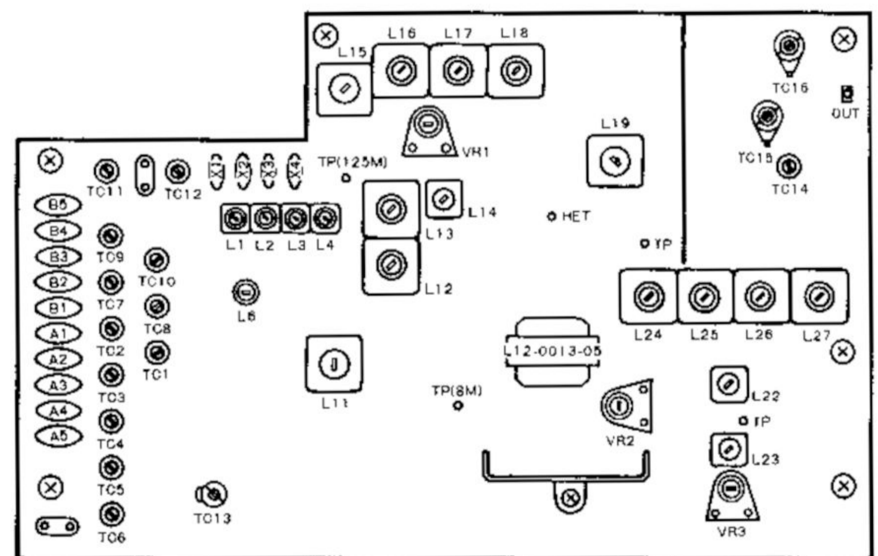
FIG. 2 SYNTHESIZER UNIT
