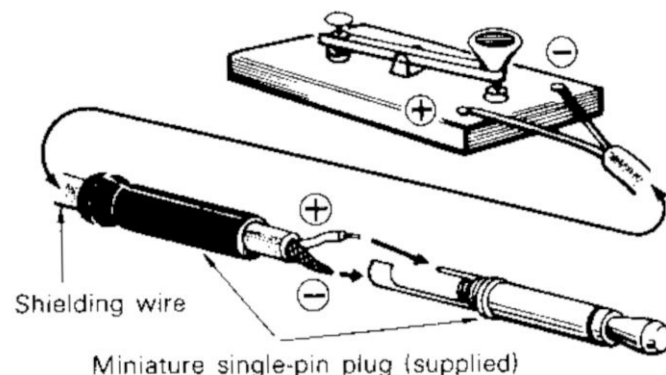
FIG. 22 KEY CONNECTION
