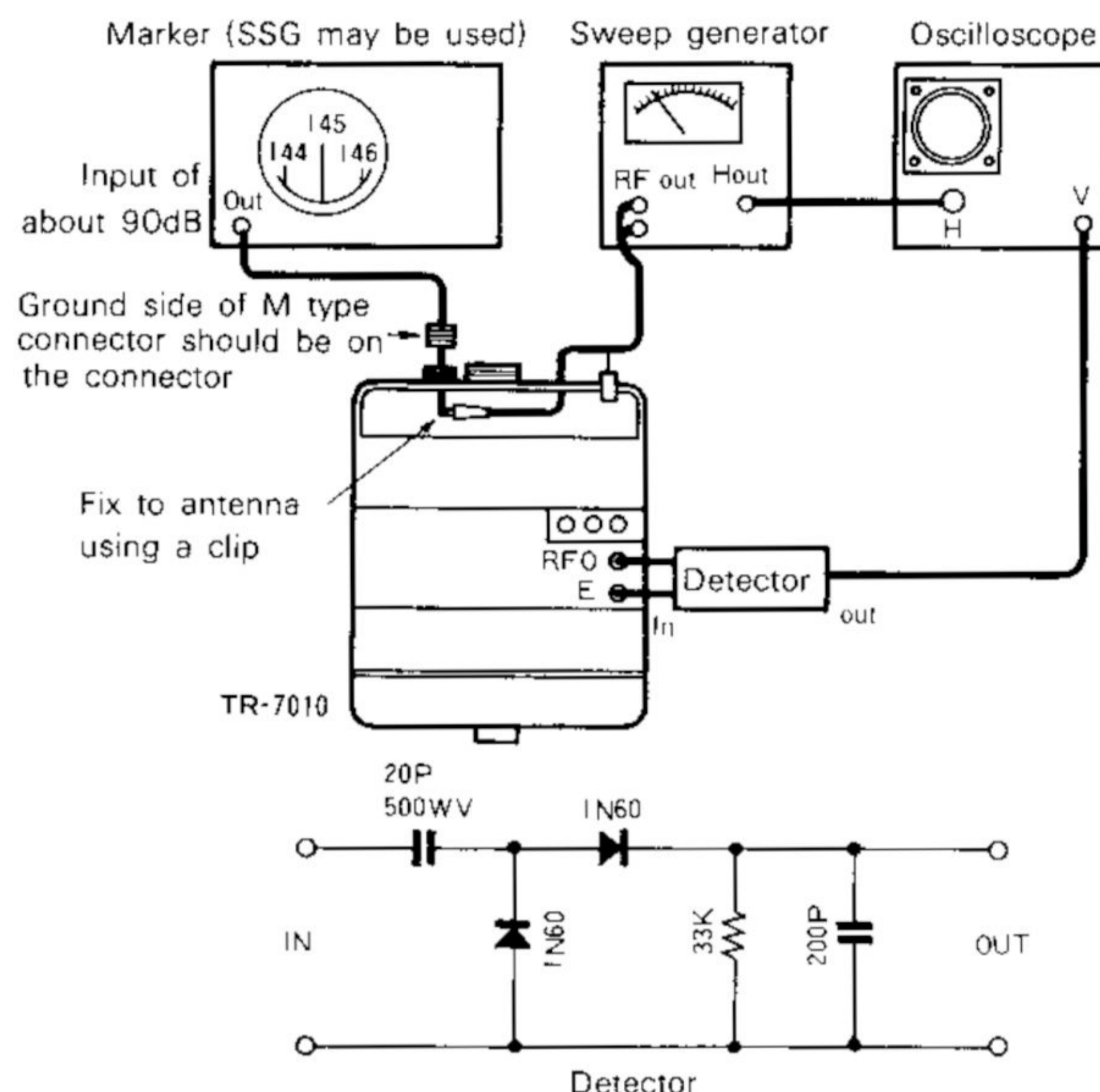
FIG. 12 HELICAL ADJUSTMENT
