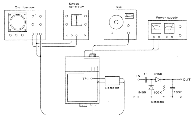
Fig. 7 RF Circuit Adjustment
