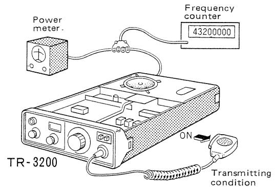
Fig. 16 Frequency Adjustment
