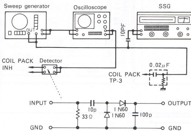
Fig. 40-b TX BPF adjustment
