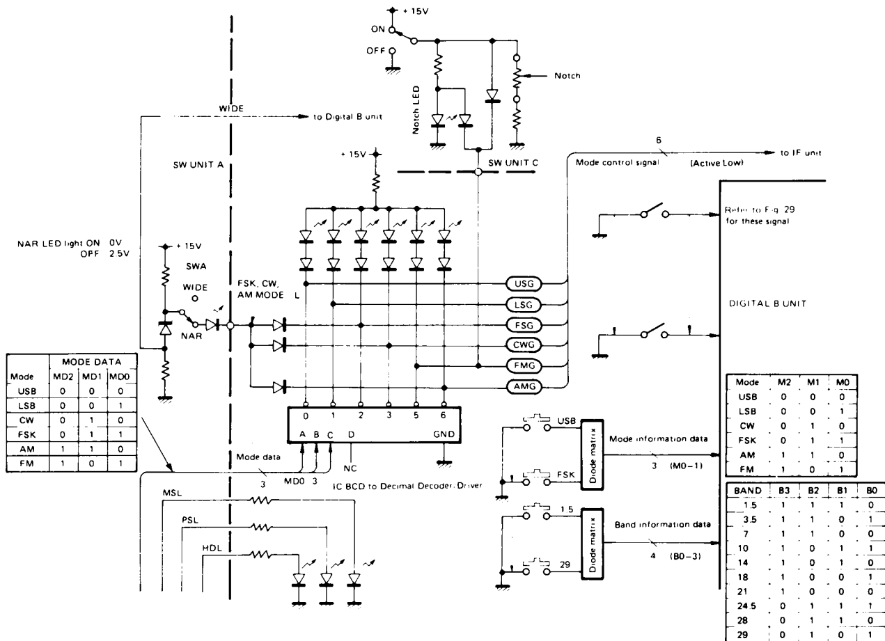
Fig. 50 Keyboard assy
