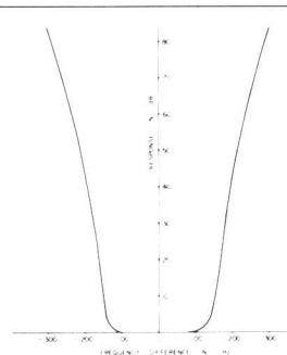
YG-455C-1 characteristic
