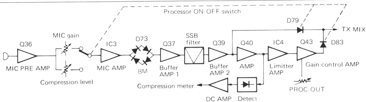
Fig.-19 A block diagram of the speech processor
