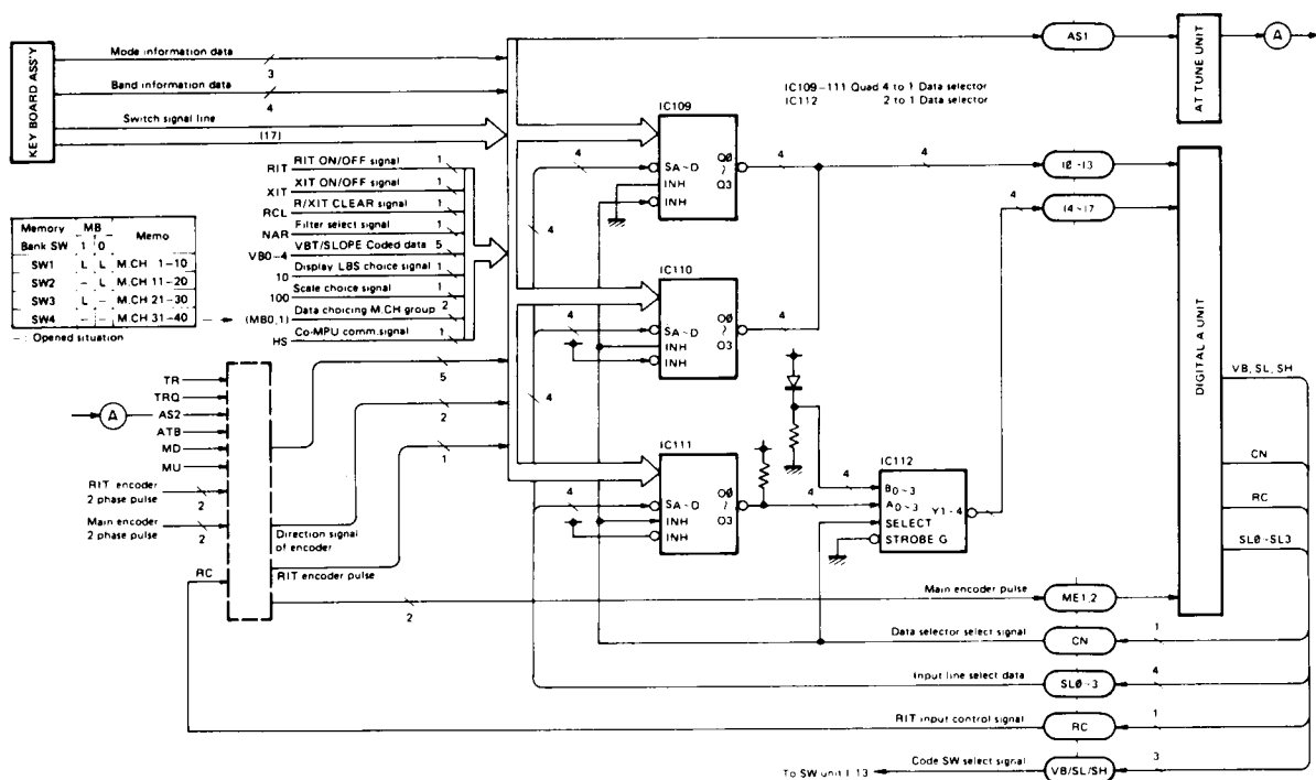
Fig.-43 Digital B unit block diagram
