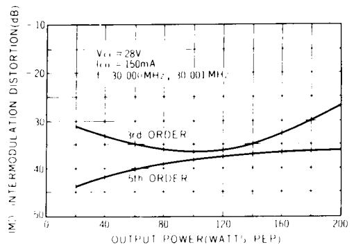
Fig.-36 (b) MRF422 intermodulation distortion versus output power
