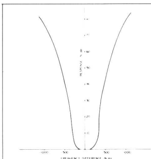
Fig.-52(a) YK-88C-1 characteristic
