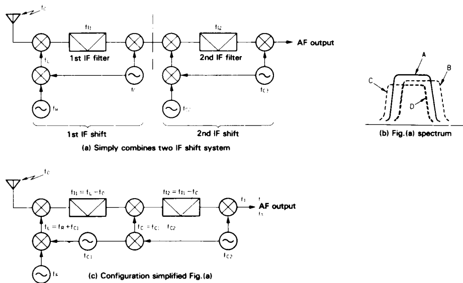
Fig.-11 Variable bandwidth theory
