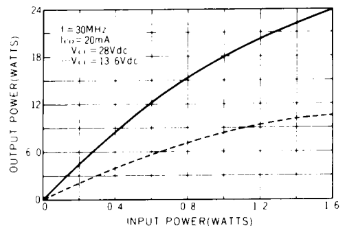
Fig.-37 (a) MRF485 output power versus input power
