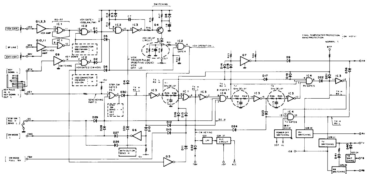
Fig.-25 Timing circuit basic configuration
