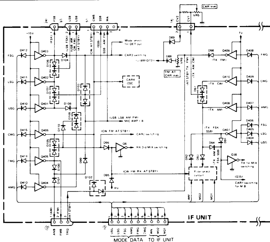
Fig. 51 Mode selector signal block diagram
