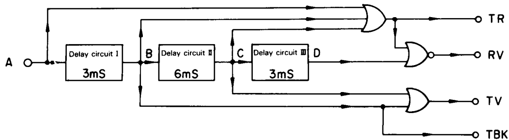
Fig.-25 Timing circuit basic configuration
