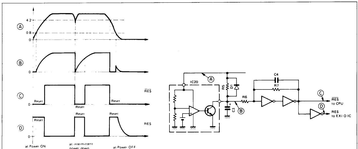
Fig.-46 Reset circuit
