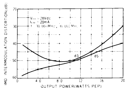
Fig.-37 (b) MRF485 intermodulation distortion versus output power
