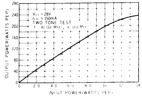
Fig.-36 (a) MRF422 output power versus input power
