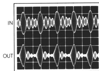
Fig.-20 The speech processor's effect (Approx. 10 dB compression)
