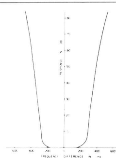
YG-455CN-1 characteristic
