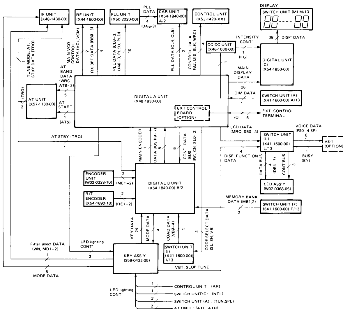
Fig.-42 Digital control block diagram
