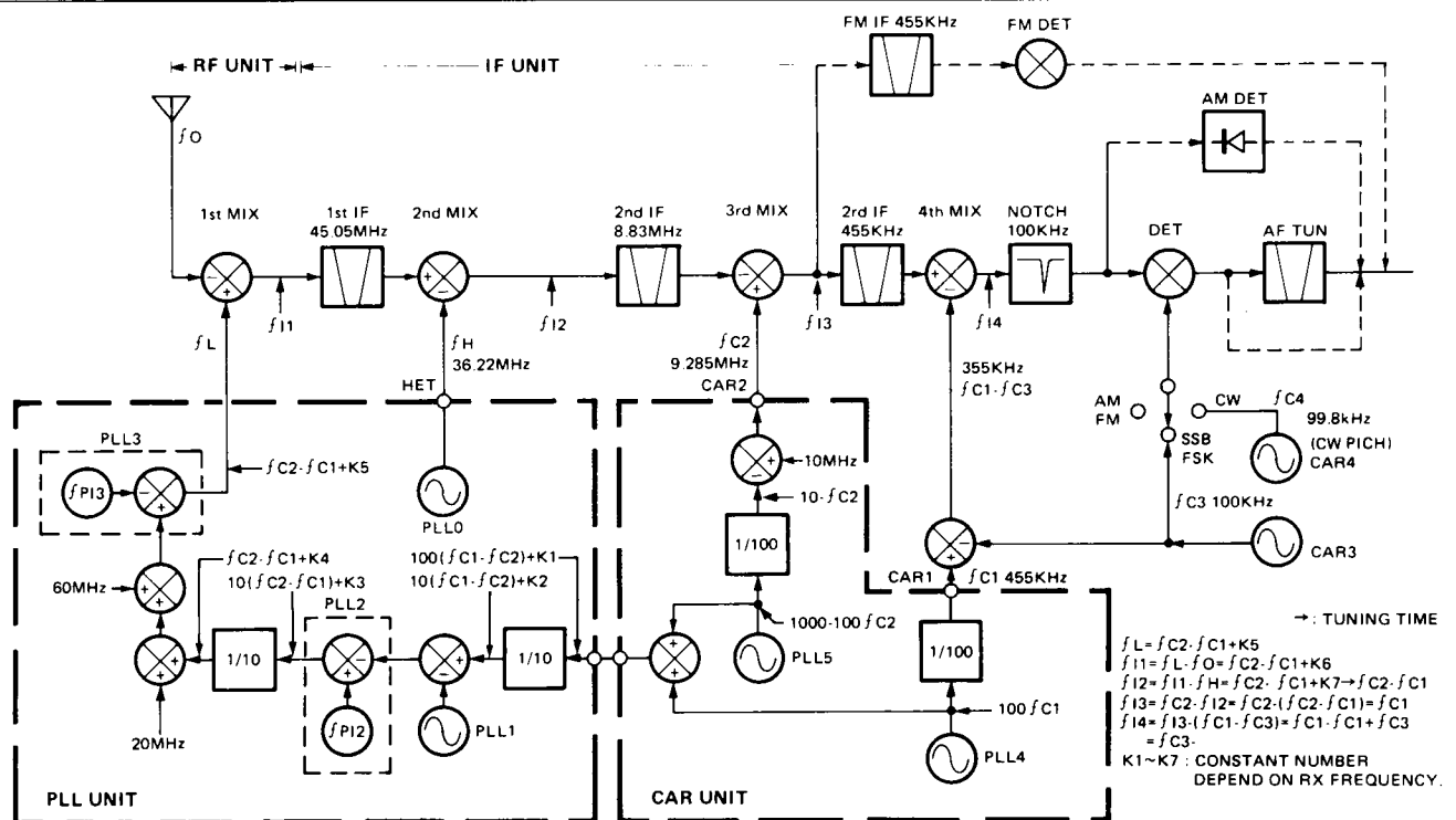
Fig.-12 RX configuration normal (wide) response
