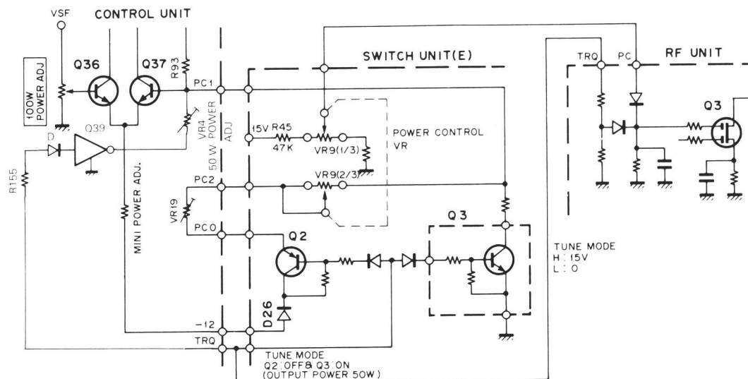
Fig.-18 Power control circuit
