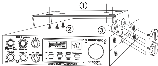
MOUNTING DIAGRAM
