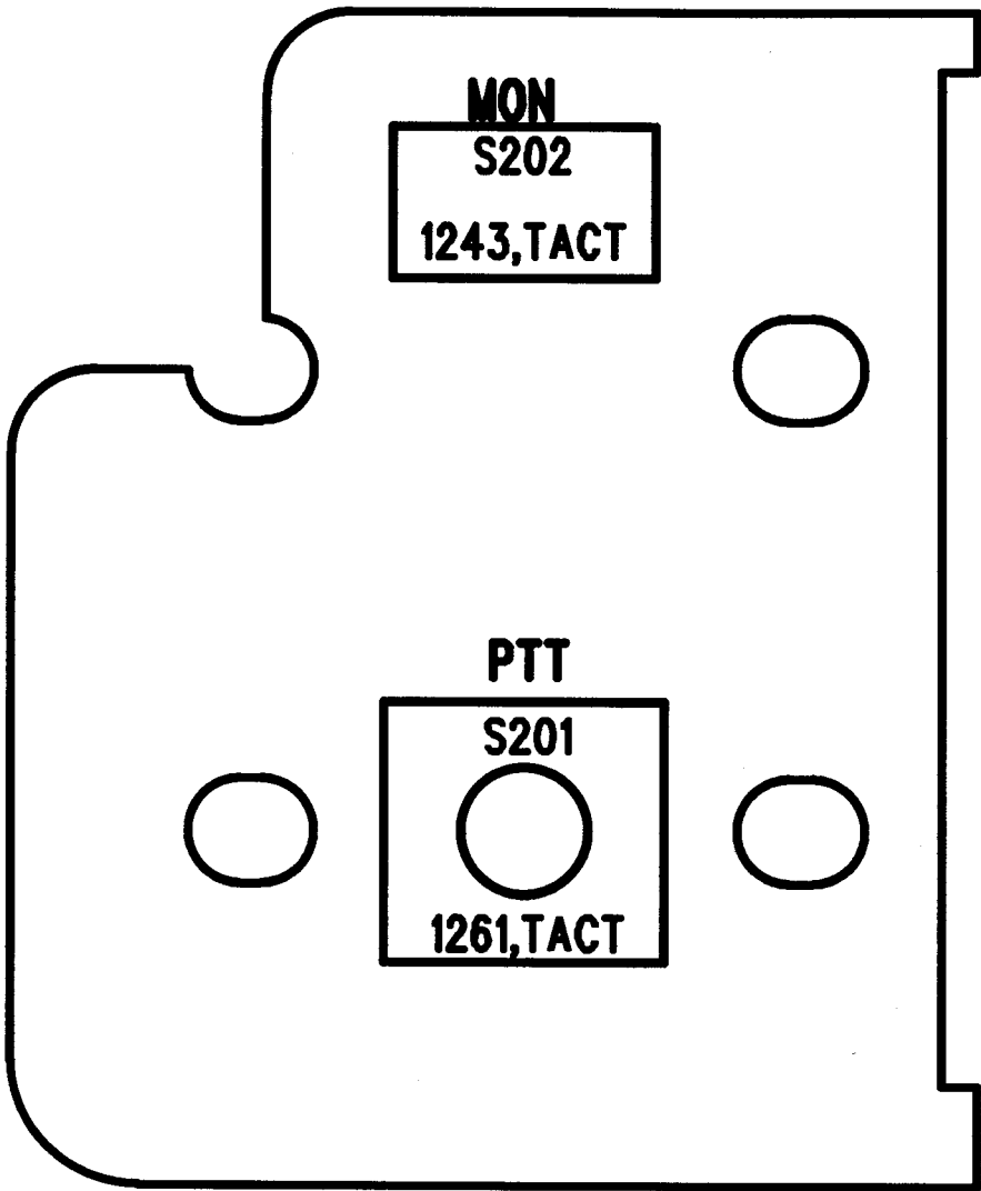
TOP SILK SCREEN
