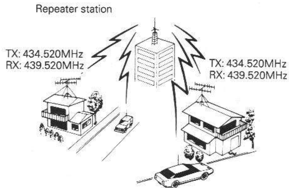
Repeater operation (in case of 430 MHz band)
