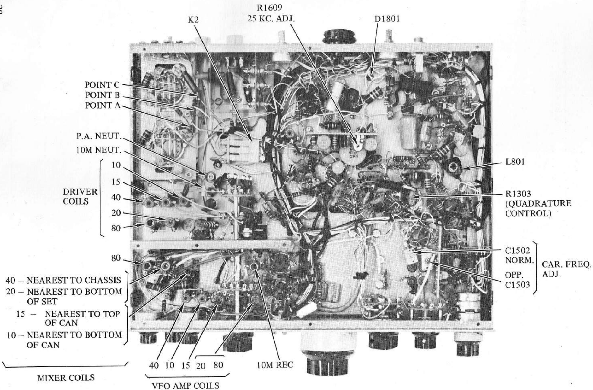
FIGURE 5. BOTTOM VIEW MODEL 700-CX
