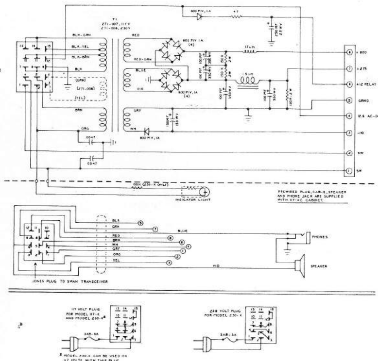
FIGURE 9. SWAN MODEL 117-X (230-X) A.C. POWER SUPPLY
