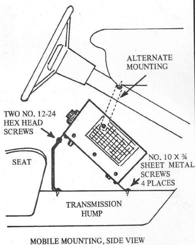
FIGURE 3. MOBILE MOUNTING ON TRANSMISSION HUMPH UNDER DASH
