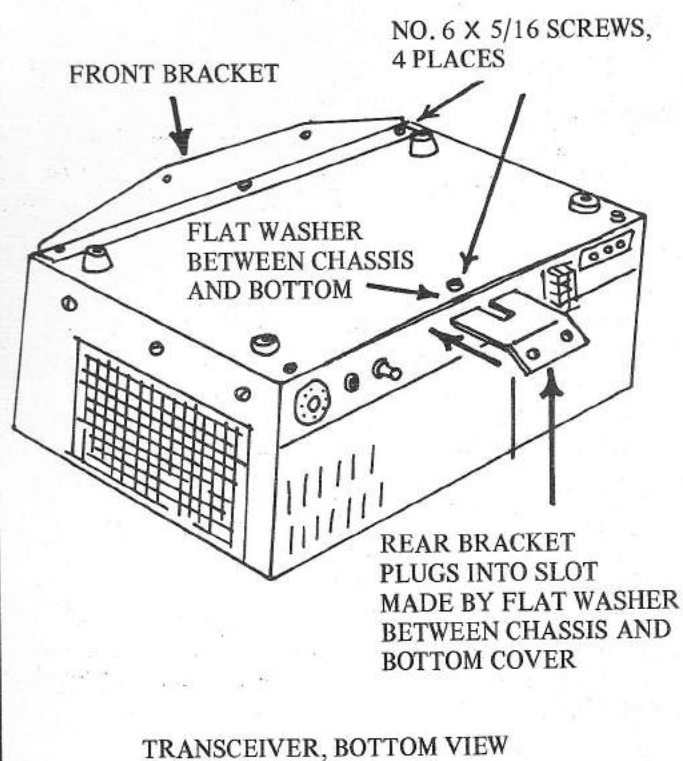
FIGURE 3. MOBILE MOUNTING ON TRANSMISSION HUMPH UNDER DASH
