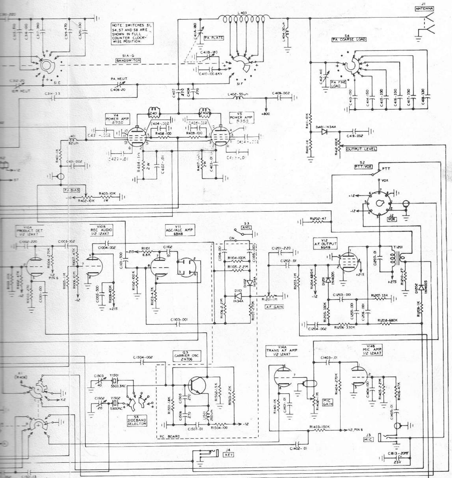
Swan Model 700CX Transceiver Schematic Diagram
