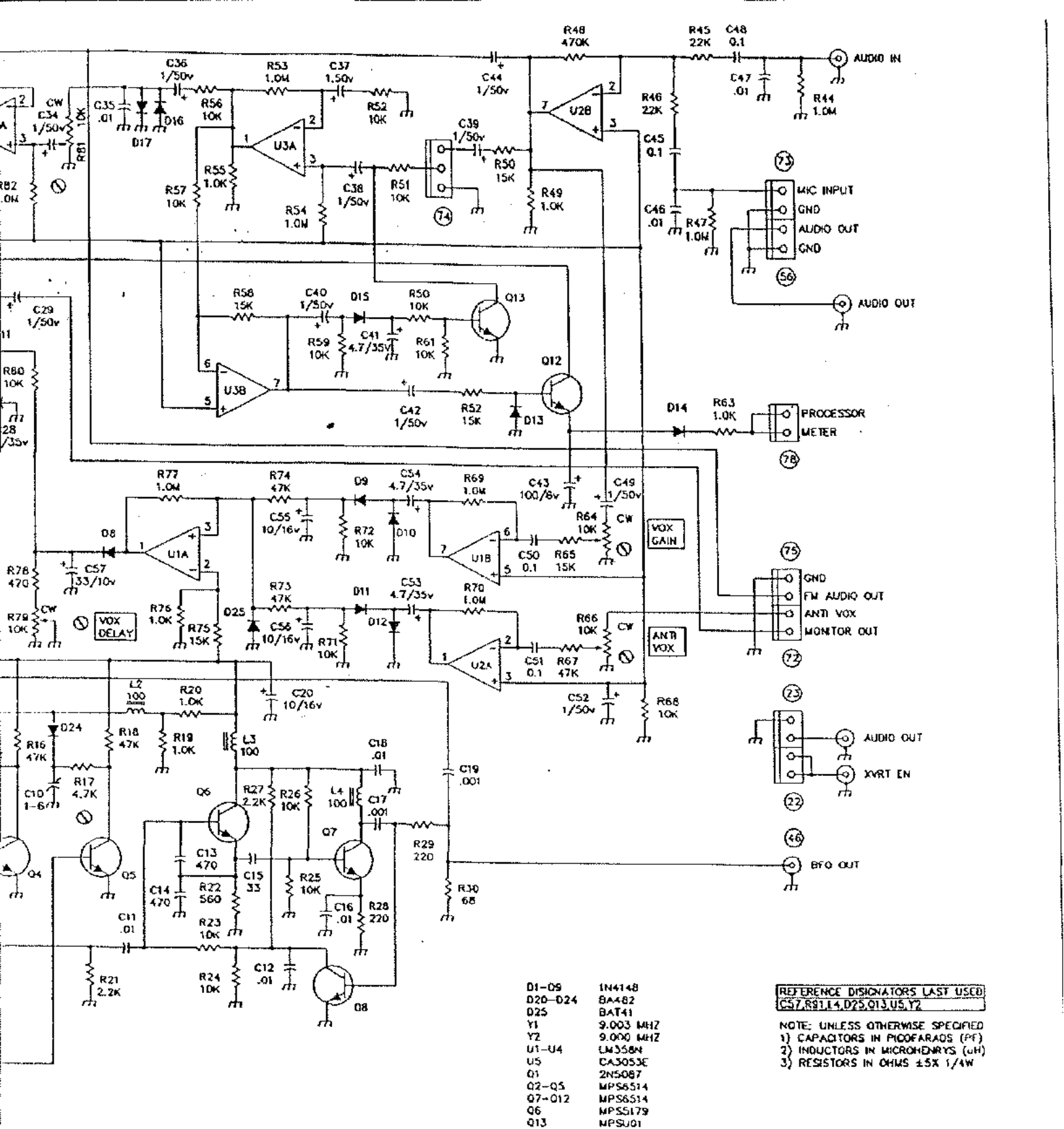
FIGURE 4-36. TX AUDIO/BFO SCHEMATIC (81634)
