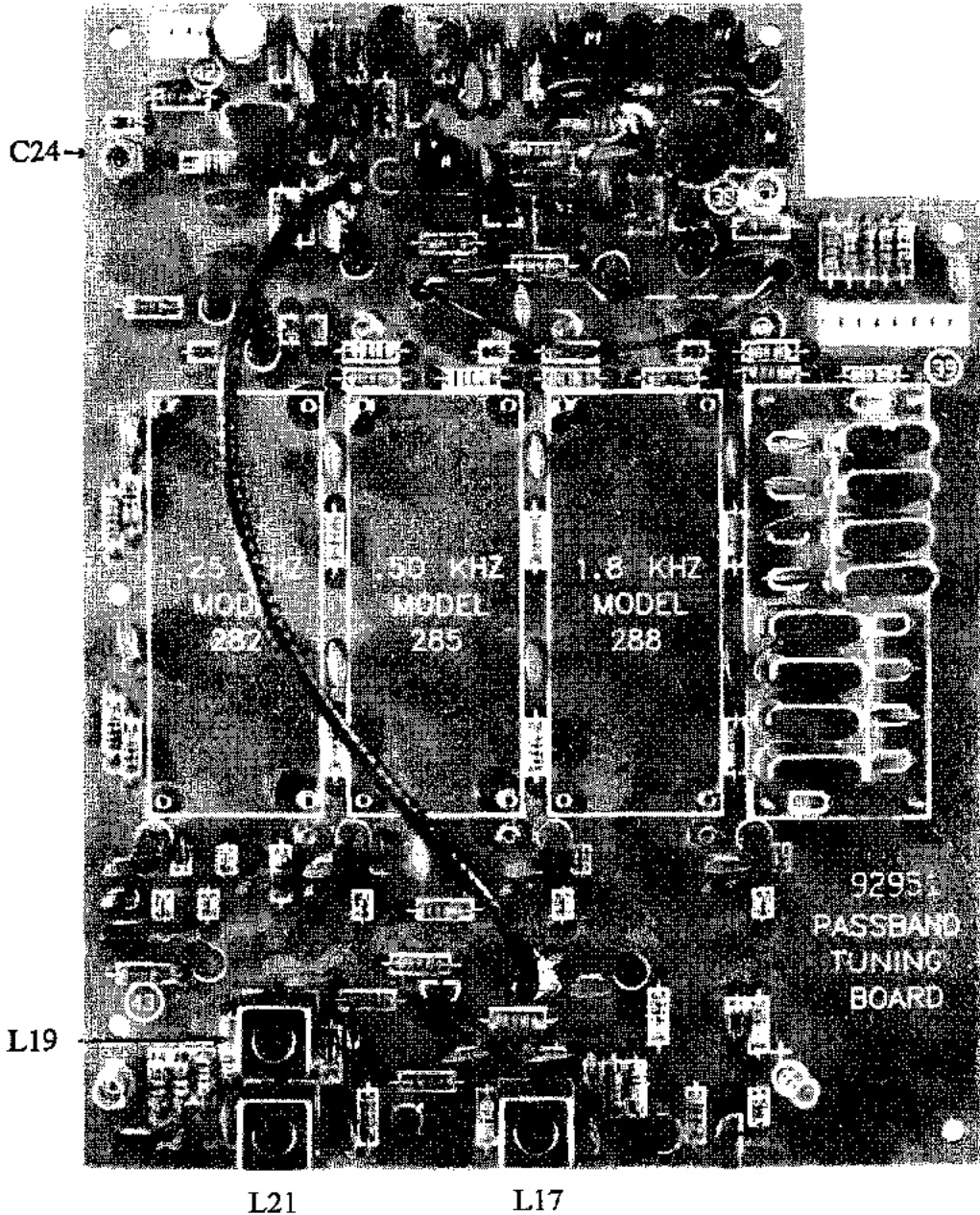
FIGURE 4-29. PASSBAND TUNING BOARD COMPONENT LAYOUT (81631)
