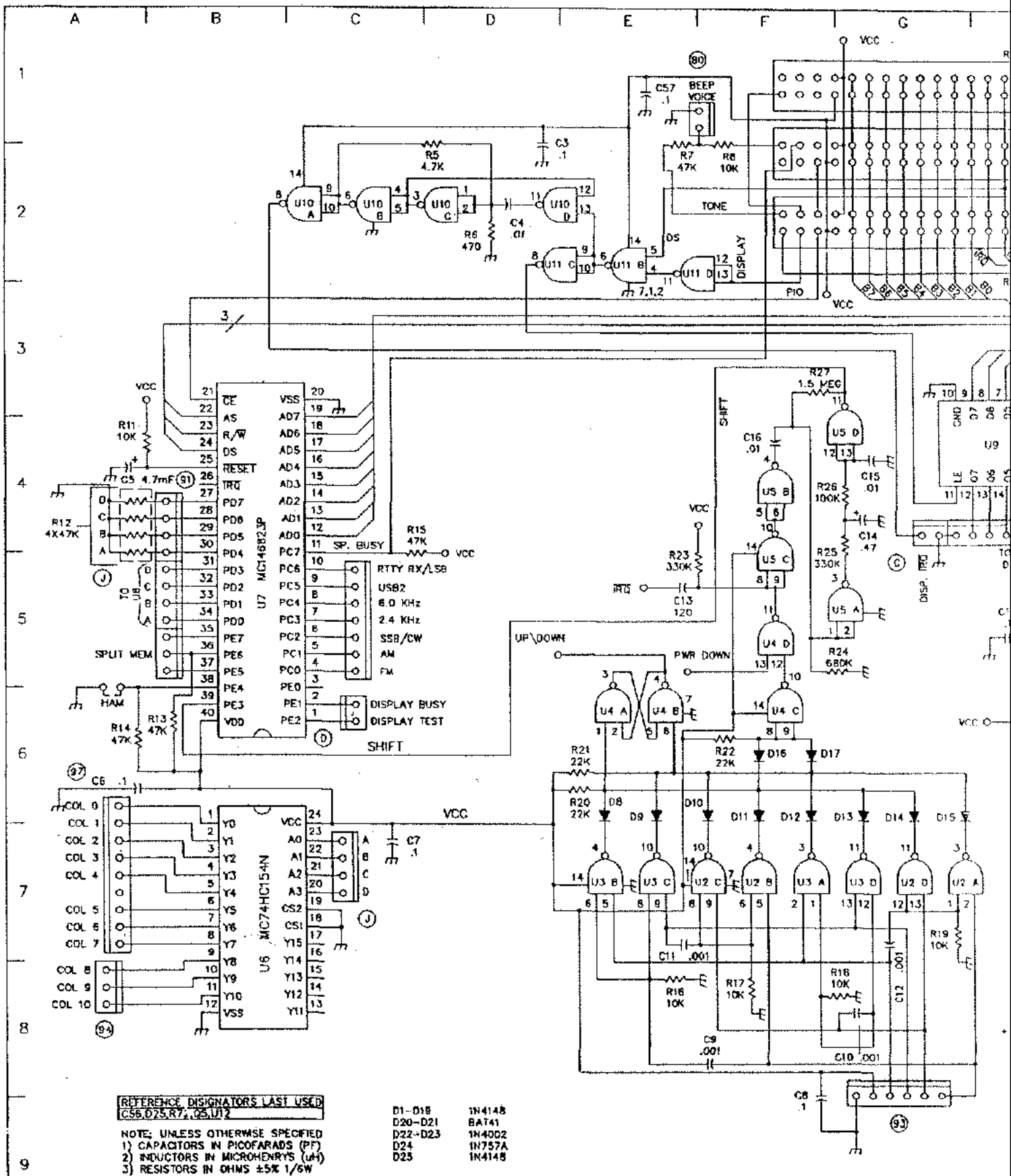
FIGURE 4-2. LOGIC BOARD SCHEMATIC (8)
