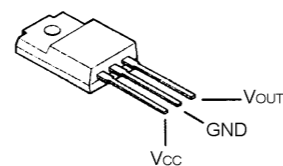
BAJ2CC0T (Lot.1-4) (Q5405)
