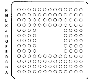
Bottom View TMS320C6713BZDP (Q7519)
