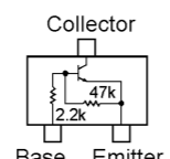
DTC123JE (E42) (Q5402)
