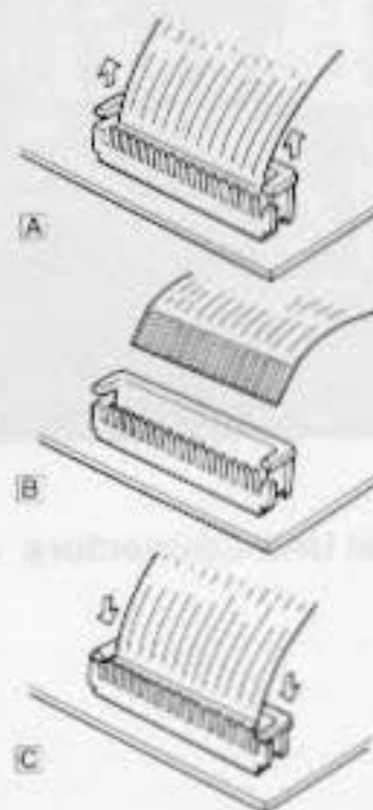
Figure 3: Ribbon Cable Connector
