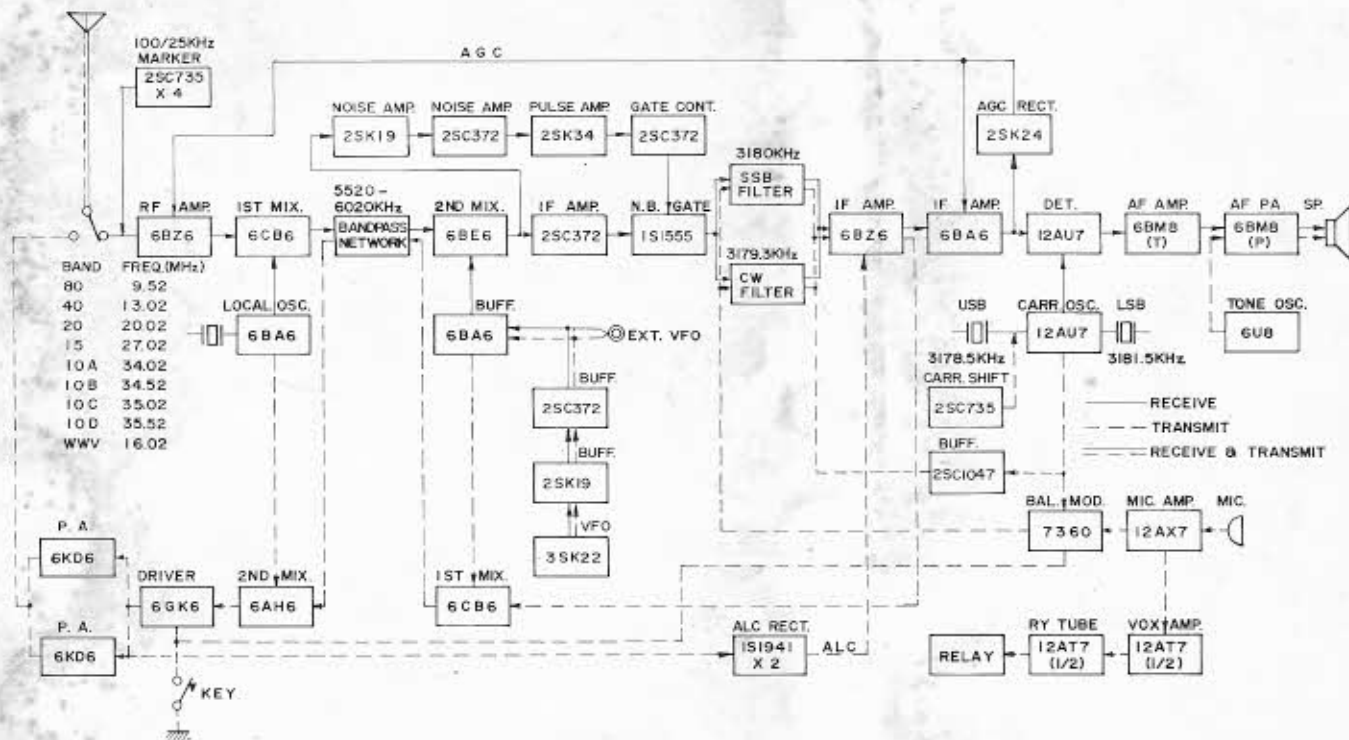
BLOCK DIAGRAM
